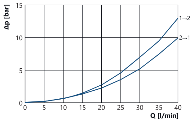
Pressure loss characteristic curve ( \Delta p/Q ) MSVT-22
