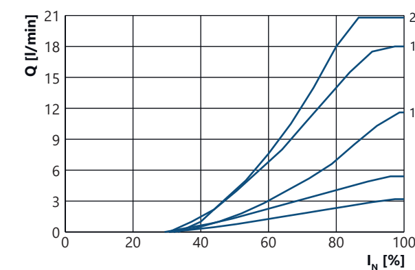
Flow rate diagram (Q/I) EPSR2-11
