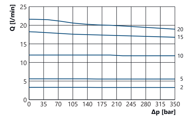
Flow rate diagram (Q/p) EPSR2-11
