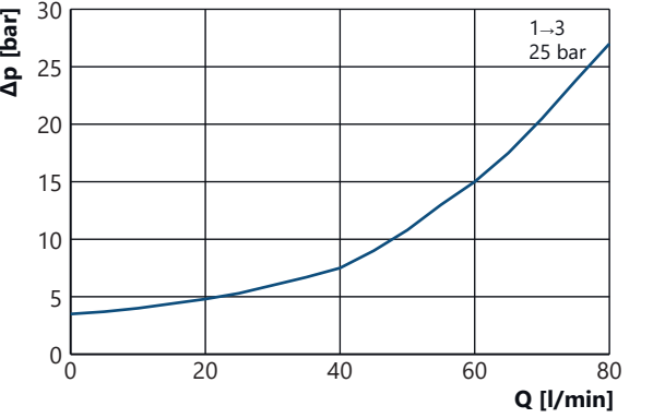
Pressure loss characteristic curve ( \Delta p/Q ) EPDRS3-10 at I = 0 mA (deenergized)
