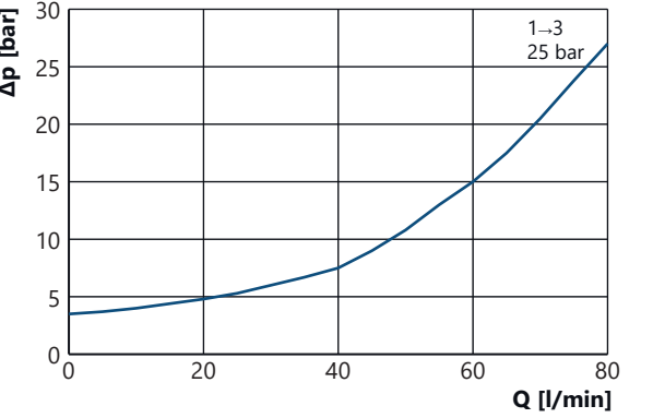
Pressure loss characteristic curve ( \Delta p/Q ) EPDRS3-10 degressive version at I = 100 % (full current)
